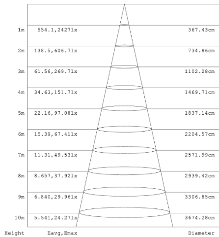
Diagram for RSBEX18-01 in 65W, 4000K. Other diagrams available on request
