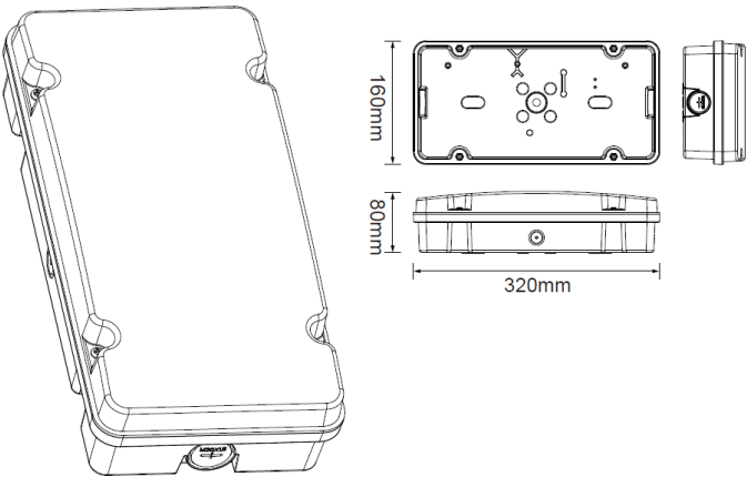
Dimension Diagram
