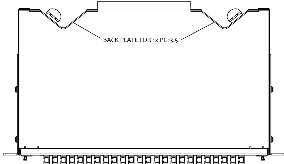
ODF BOX TOP VIEW A
