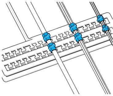
FIST External cable fixation bracket for GC02-FX fiber closure
