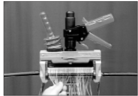
5. Remove excess wire from module by lifting groups of conductors straight up from retainer spring and pulling gently.
