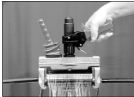
4. Pump handle until module is crimped and pressure by-pass operates.
